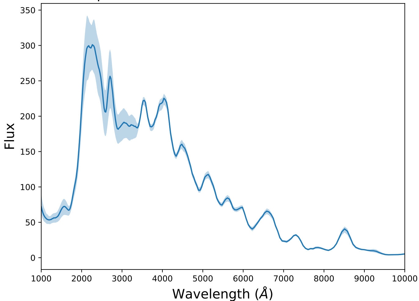
Spectrum 7 for transient CCSN at z=1.59
